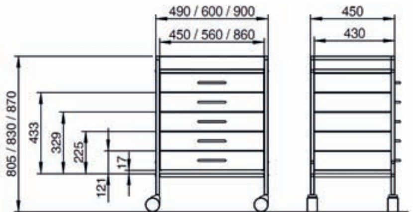
Basic trolley 805 / 830 / 870 mm high
